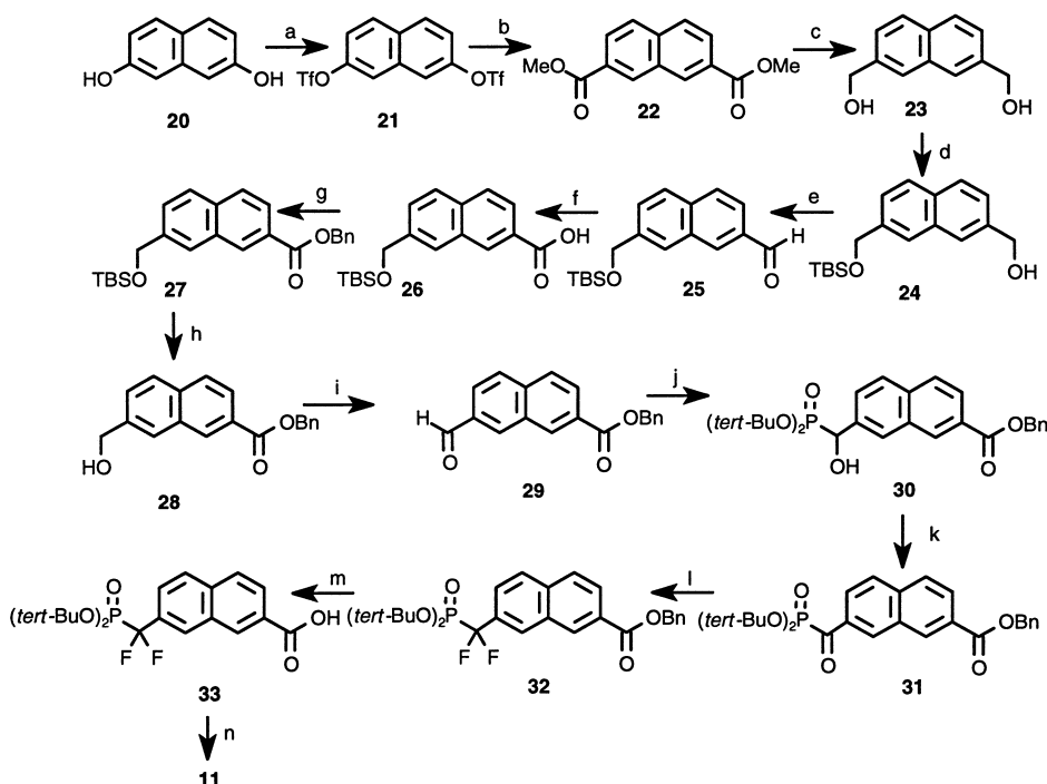
Scheme 2. Reagents and conditions: (a) \text{TiCl}_4 , 2,6-lutidine, DMAP, \text{CH}_2\text{Cl}_2 -THF, 74%; (b) \text{Pd}(\text{OAc})_2 , dppp, CO, MeOH, TEA, DMSO, 84%; (c) \text{LiAlH}_4 , THF, 59%; (d) \text{LiHMDS} , TBDMSCl, 45%; (e) \text{MnO}_2 , toluene, 77%; (f) \text{NaClO}_2 , \text{KH}_2\text{PO}_4 , 2-methyl-2-butene, t\text{-BuOH} -water, 98%; (g) DBU, BnBr, DMF, 92%; (h) TBAF, THF, 93%; (i) PCC, \text{CH}_2\text{Cl}_2 , 95%; (j) (t\text{-BuO})_2\text{P}(\text{OH})\text{H} , \text{LiHMDS} , THF, 98%; (k) Swern oxidation, 71%; (l) DAST, 52%; (m) 0.2 N LiOH, THF; (n) DIPCDI, HOBT, NMP; TFA, anisole; HPLC, 30%.
