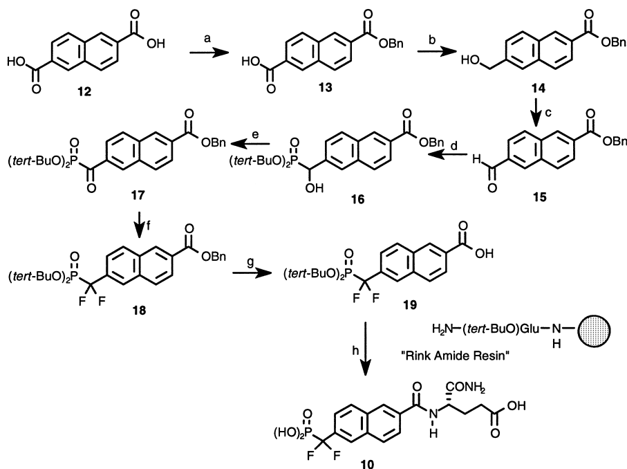
Scheme 1. Reagents and conditions: (a) DBU, BnBr, DMF, 17%; (b) BH 3 ·THF, THF, 84%; (c) MnO 2 , toluene, 100%; (d) (t-BuO) 2 P(O)H, basic Al 2 O 3 , 91%; (e) Swern oxidation; (f) DAST, 59%; (g) 0.2 N LiOH, THF, 74%; (h) DIPCDI, HOBT, NMP; then TFA, anisole; HPLC, 44%.
